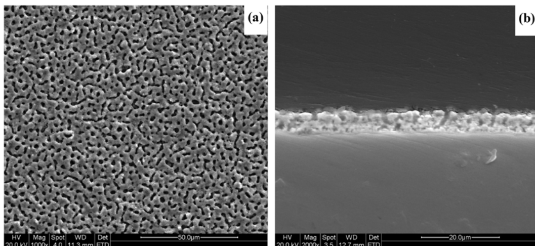
Fig. 1. Morphologies of \text{WO}_3/\text{TiO}_2 composite film: (a) surface morphology; (b) cross-section morphology.
